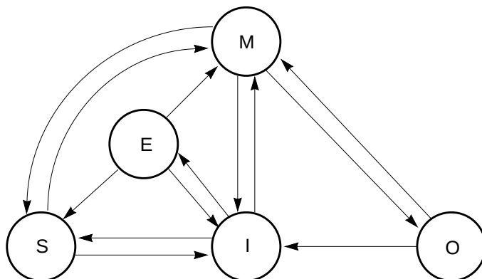
Figure 7-20 Cache Coherency Protocol State Diagram
