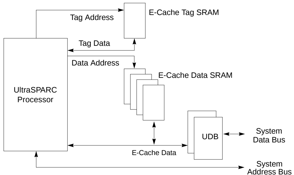
Figure 1-2 UltraSPARC Subsystem
