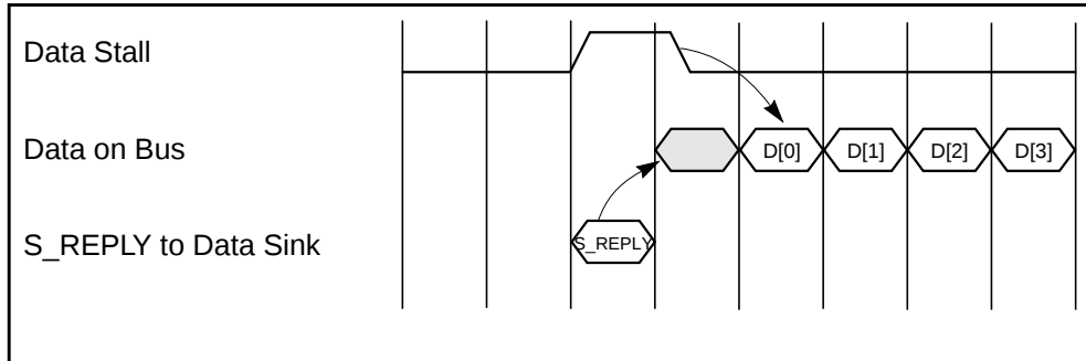
Figure 7-30 Data_Stall to UltraSPARC Sinking Data
