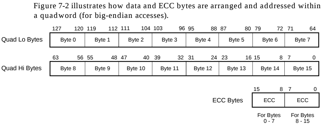
Figure 7-2 Data and ECC Byte Addresses Within a Quadword
