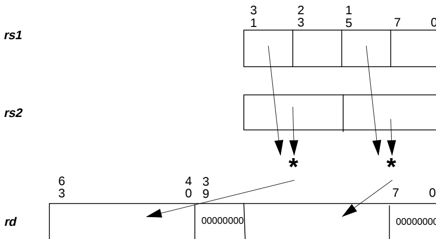
Figure 13-13 FMULD8SUx16 Operation
