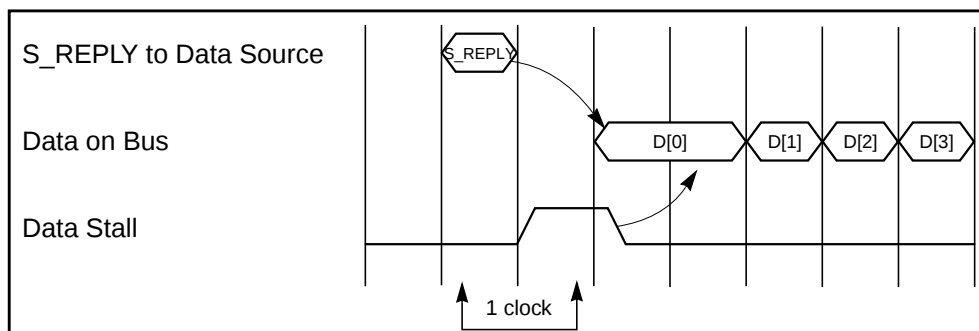
Figure 7-29 Data_Stall to UltraSPARC Sourcing Data
