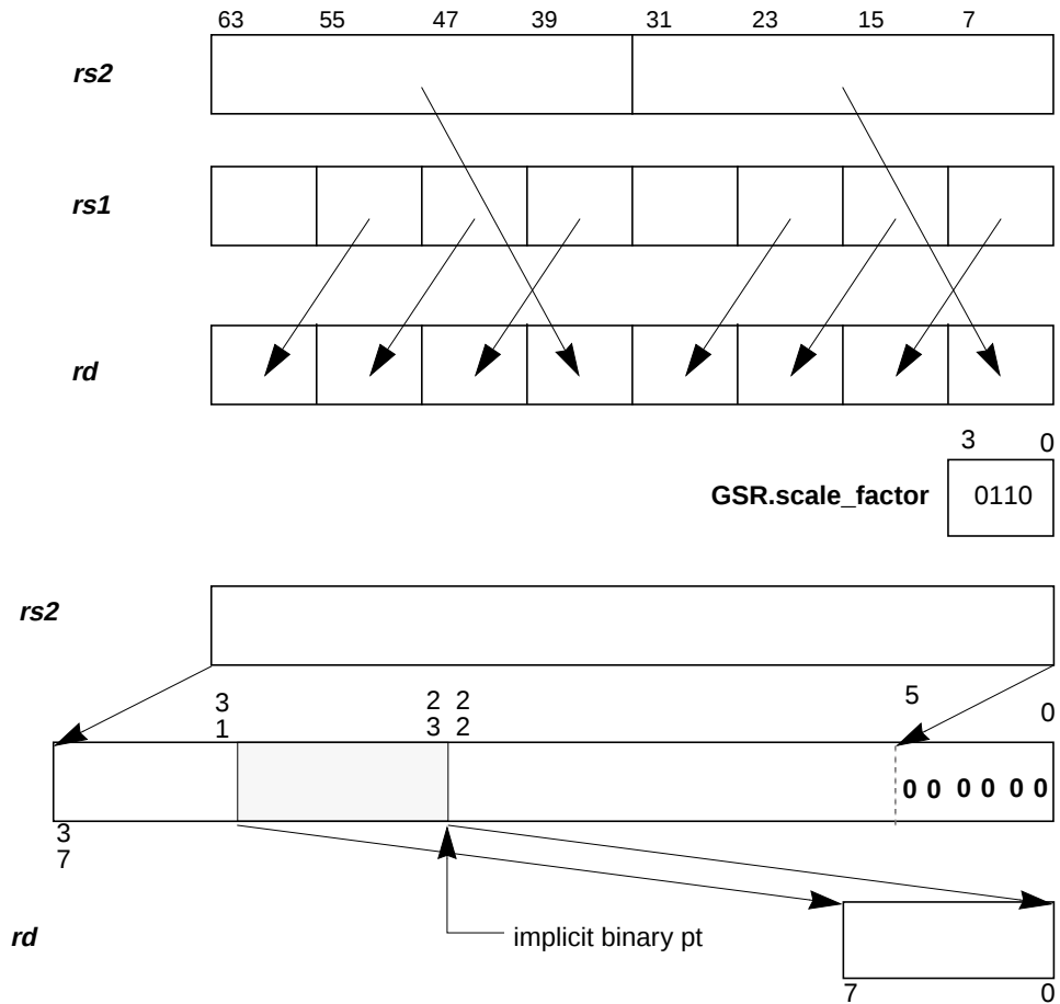
Figure 13-4 FPACK32 Operation
