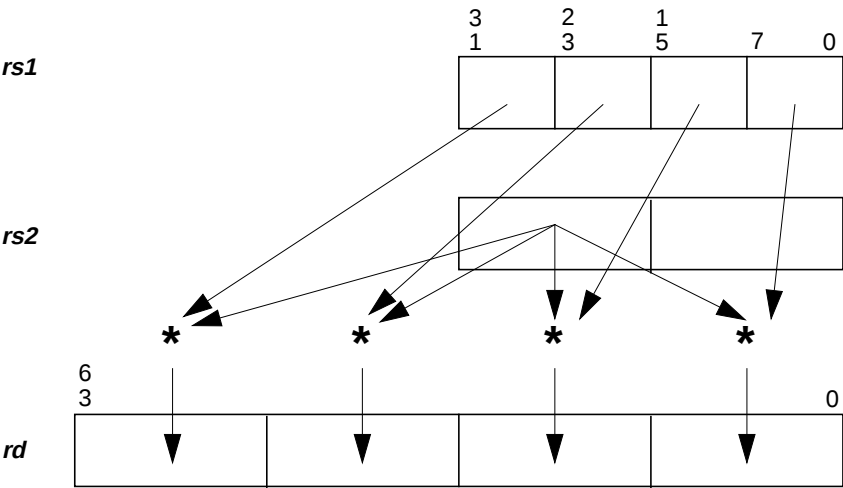
Figure 13-9 FMUL8x16AU Operation
