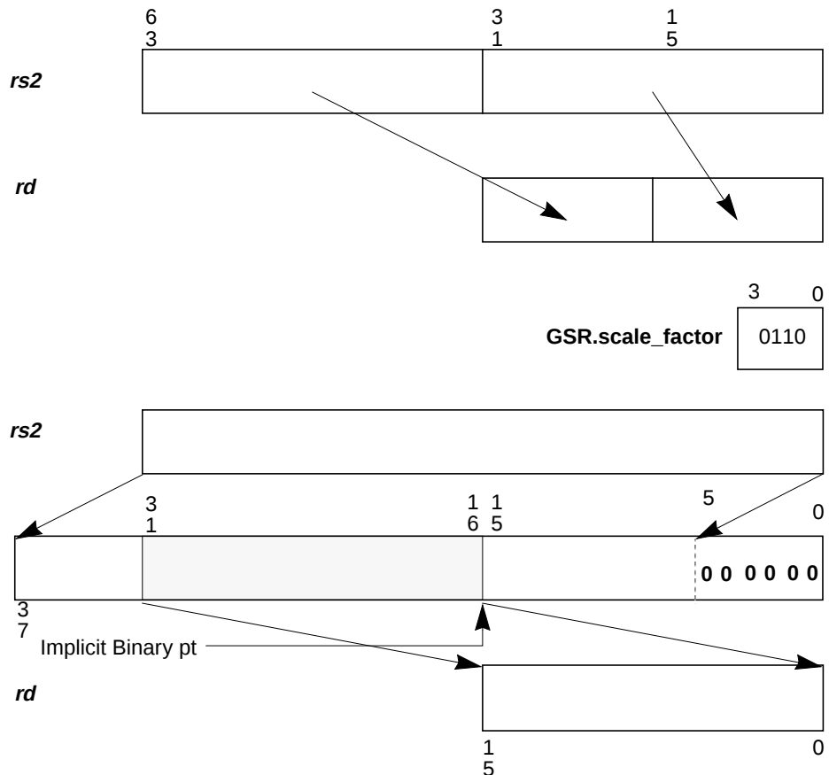
Figure 13-5 FPACKFIX Operation
