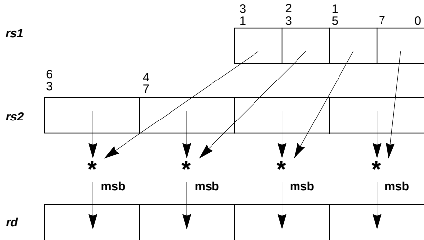
Figure 13-8 FMUL8x16 Operation
