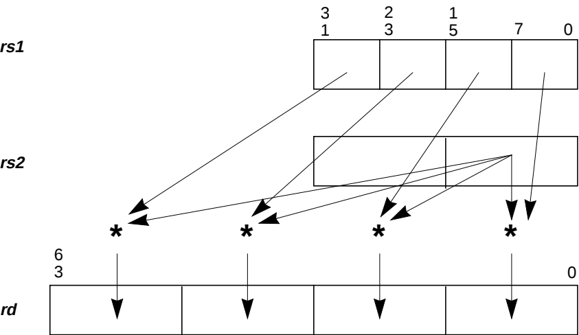
Figure 13-10 FMUL8x16AL Operation
