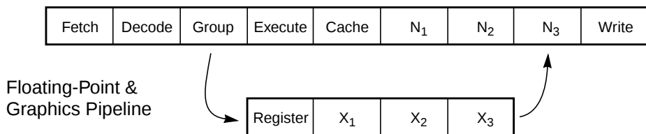
Integer Pipeline
