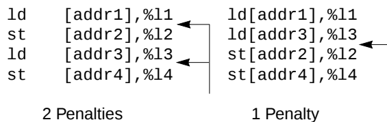
Code Example 16-3 Avoiding Bus Turnaround Penalties (1–1–1 mode only)
