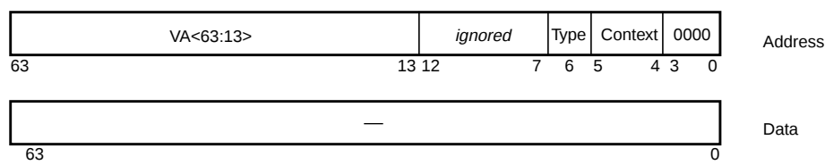
Figure 6-15 MMU Demap Operation Format
