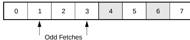
Figure 16-2 Odd Fetch to an I-Cache Line
