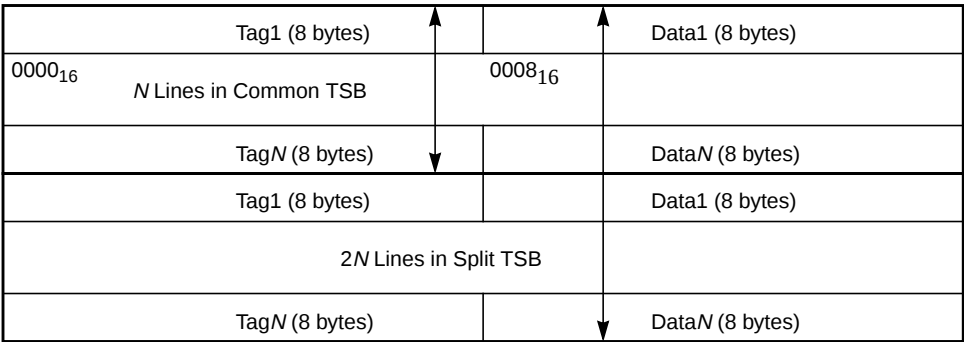
Figure 6-2 TSB Organization
