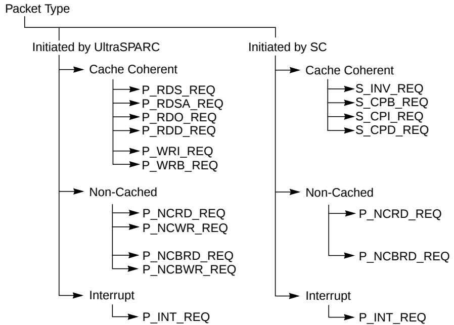
Figure 7-31 Transaction Types
