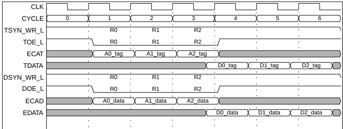
Figure 7-3 Timing for Coherent Read Hit (1–1–1 Mode)
